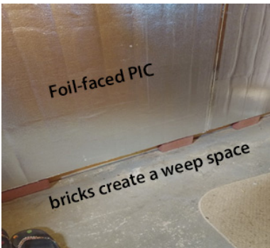
PIC foundation insulation: Installers glue PIC-foam sheets to the concrete wall, and they leave a weep space at floor level.
