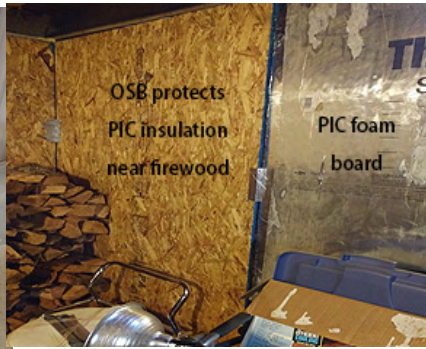
Protecting PIC foam: Installers attach OSB to protect PIC-foam sheets from firewood storage.
