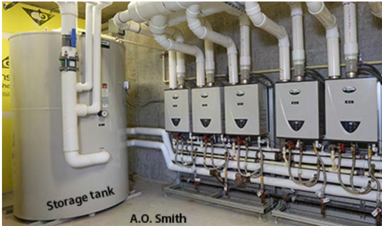
Popular multifamily water-heating solution: On-demand water heaters heat water for a storage tank and for demand in a medium-sized multifamily building.
